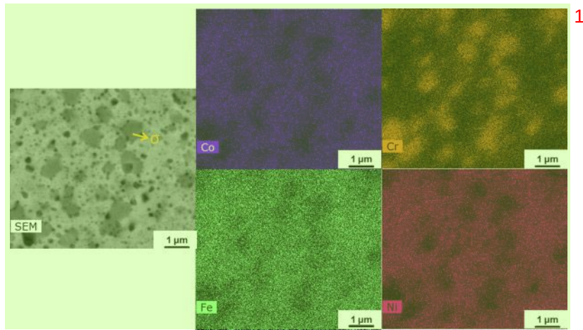
6 EDS mapping results for CoCrFeNi (SPS A ) reveal that sigma phase is rich in Cr, while the matrix is Cr depleted 2
