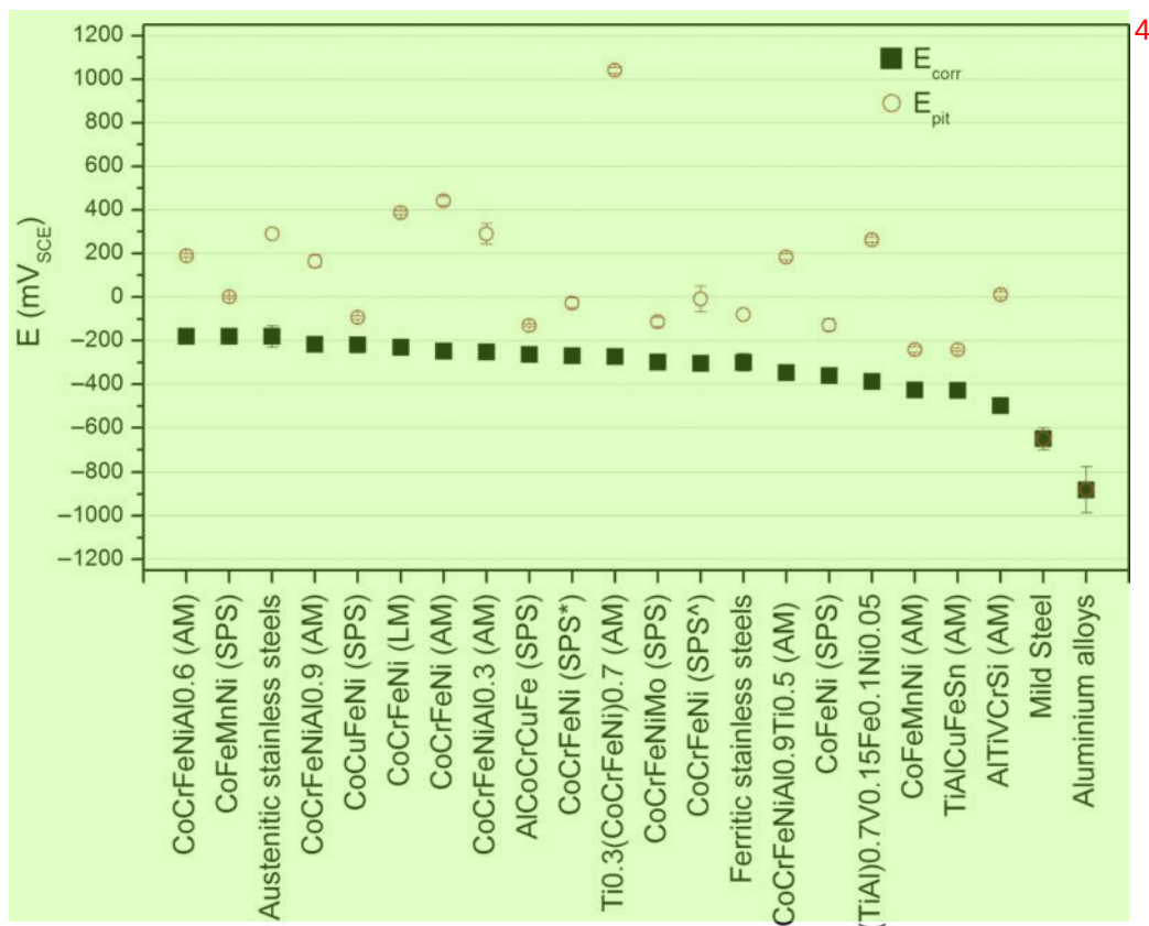
1 Summary of HEA corrosion potential ( E_{\text{corr}} in \text{mV}_{\text{SCE}} ) and pitting potential ( E_{\text{pit}} in \text{mV}_{\text{SCE}} ) in quiescent 0.6 M NaCl at 25°C; 5 CoCrFeNi (SPS*) was held at 1000°C for 5 min, while CoCrFeNi (SPS^A) was firstly held at 500°C for 5 min and then sintered at 1000°C for another 5 min; E_{\text{corr}} and E_{\text{pit}} data of steels and aluminium alloys are obtained from previous studies 24,38–39
