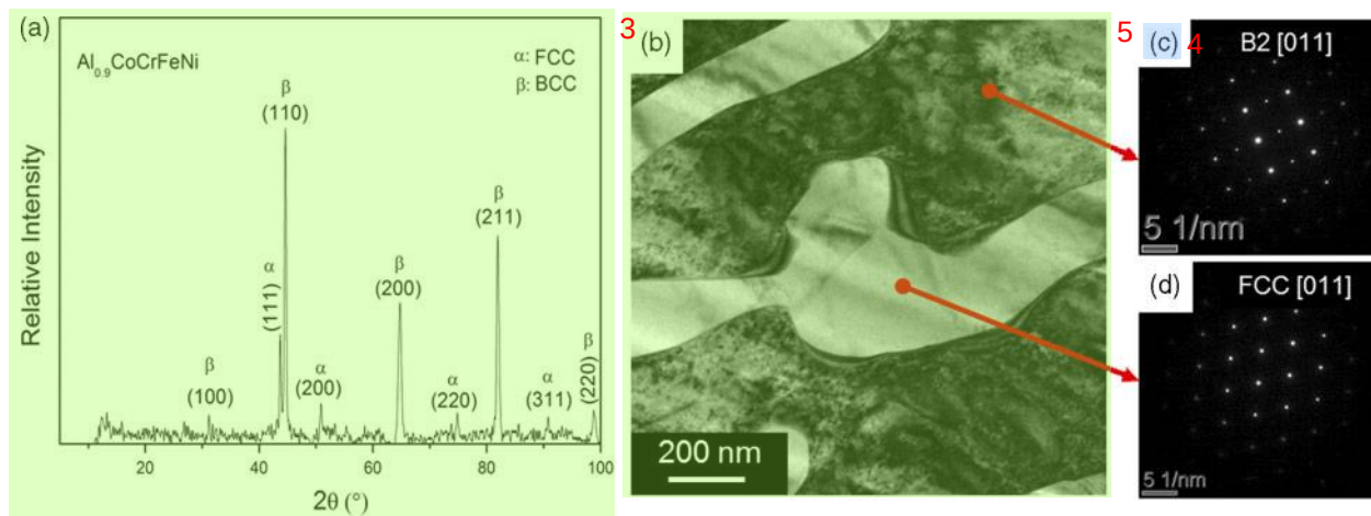
7 a XRD pattern for as cast Al 0.9 CoCrFeNi; b TEM BF image of as cast Al 0.9 CoCrFeNi; c, d SADP along [011] zone axis for 'dark' and 'light' phase respectively 6
